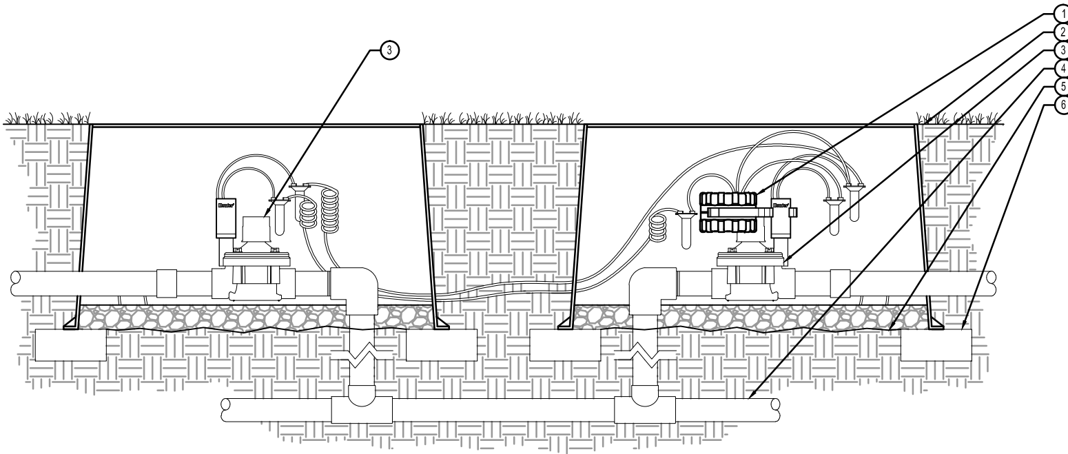
XX NODE ON VALVE WITH MULTIPLE VALVES Hunter C.NODE.03
