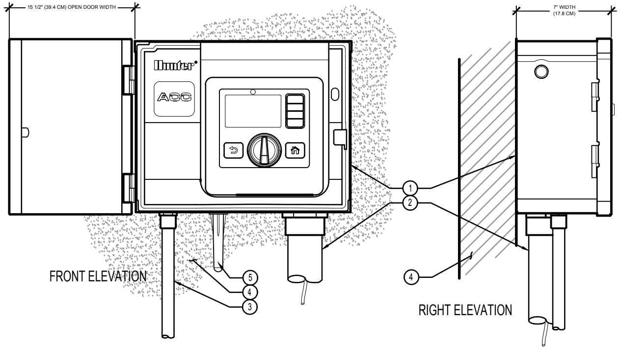
XX ACC2 DECODER - WALL MOUNT GRAY STEEL Hunter C.A2C.01
