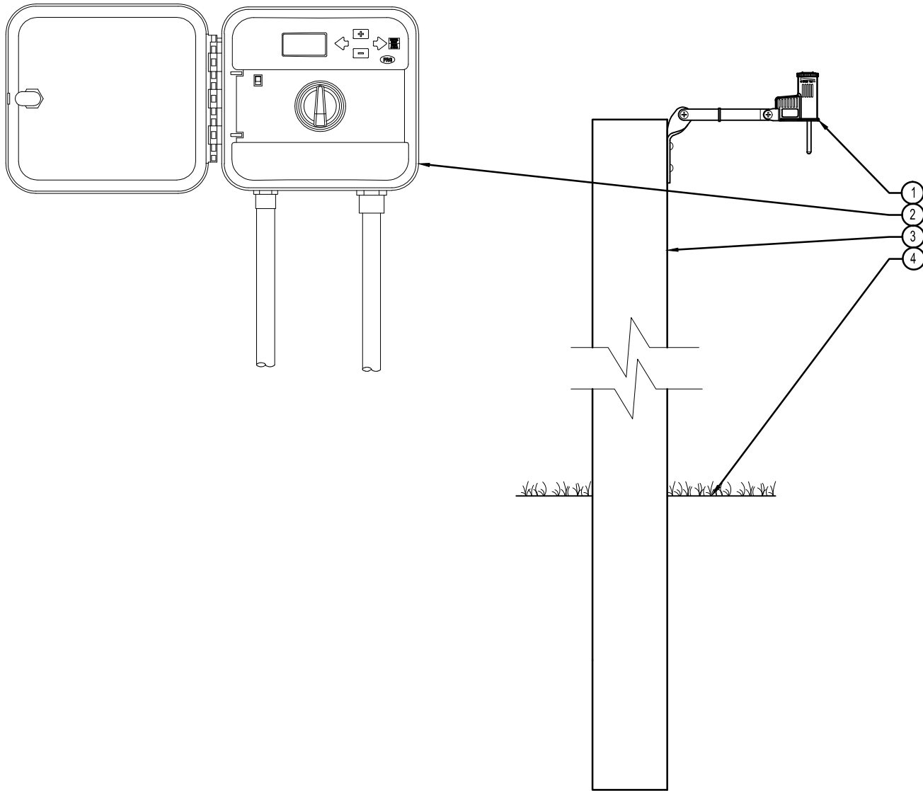
XX WIRELESS RAIN AND FREEZE CLIK WITH GENERIC WALL MOUNT CONTROLLER Hunter S.RC.08
