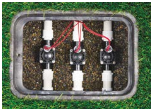
PGV-100G Valve Installed
